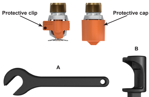
Figure 1: Sprinkler Wrenches and Protective Caps
