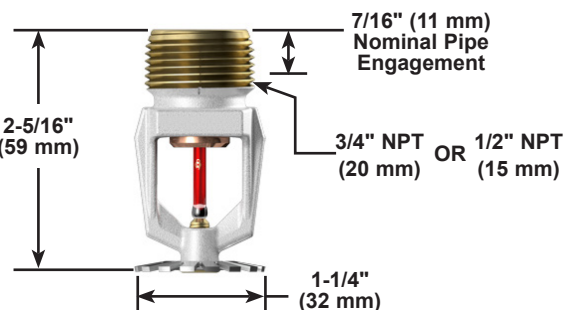
Figure 2: Sprinkler Dimensions
