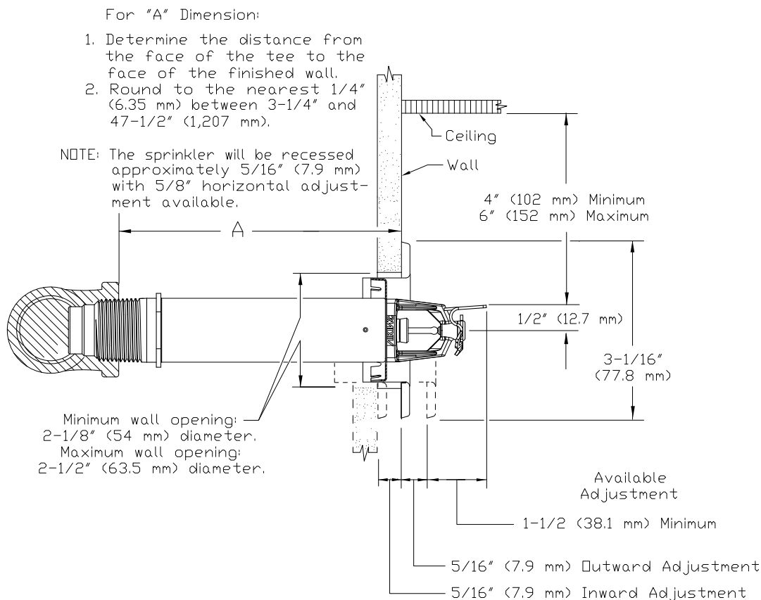
Figure 3: Adjustable Recessed Dry Horizontal Sidewall Sprinkler with the Model E-1 Escutcheon
