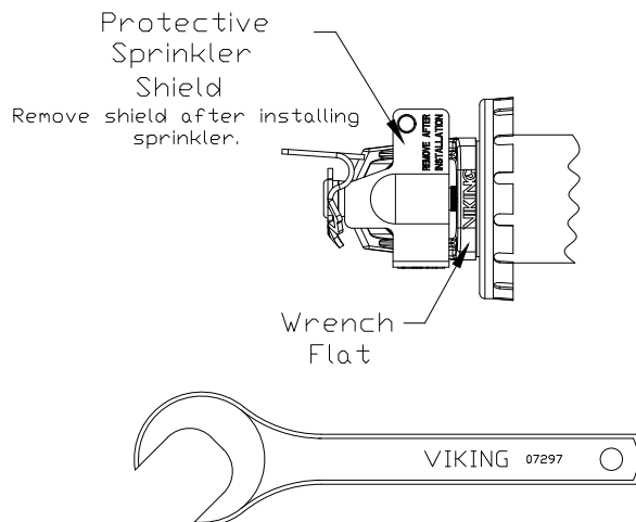
Figure 1: Sprinkler with Protective Shield
