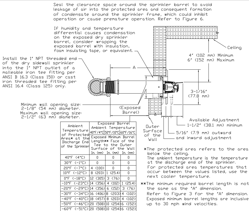
Figure 4: Dry Horizontal Sidewall Sprinkler Required Minimum Barrel Length Based on Ambient Temperature in the Protected Area
